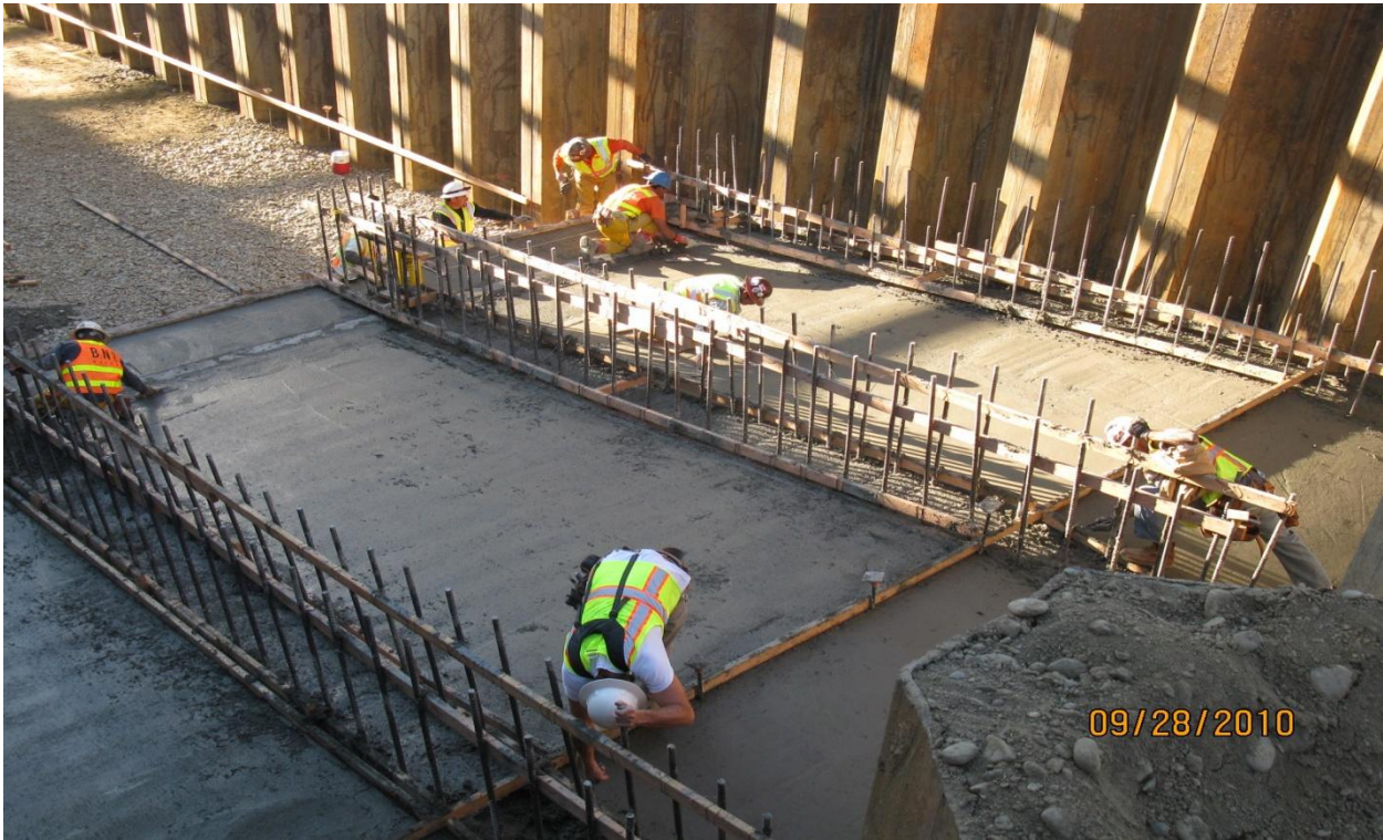
West Bay subcontractor Landavazo crew placing concrete for the siphon outlet structure slab.
